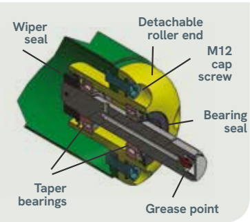
Internal roller bearings (on all MAJOR Swift and Synergy mowers)
