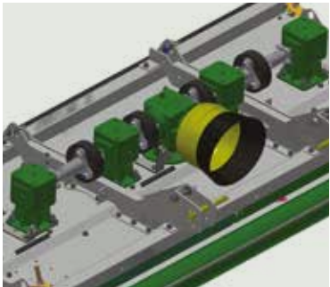
Heavy duty gearbox driven driveline
